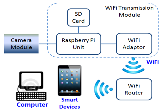
(Figure 11) Schematic diagram of WiFi-based wireless endoscope.
