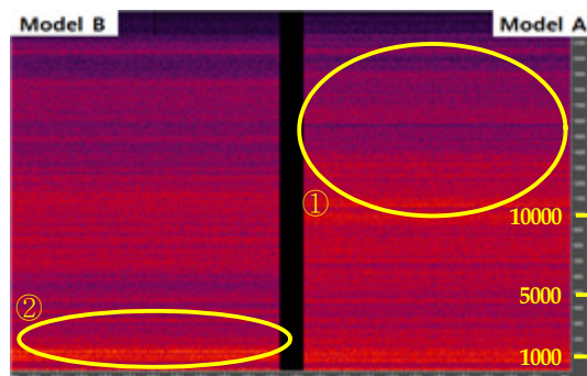
(Figure 5) Spectrogram compare between A and B
