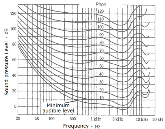
(Figure 2) Equal-loudness contour[8]
